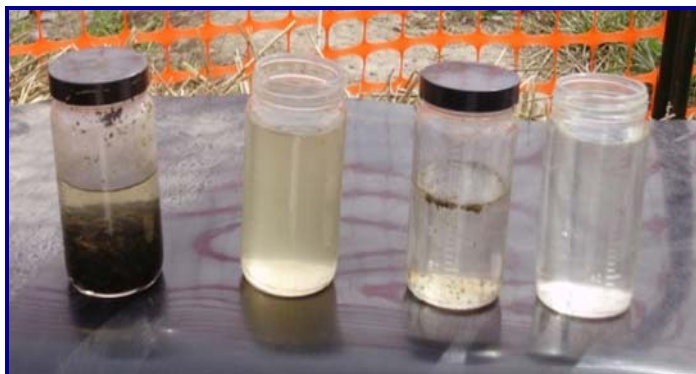
From left to right, the above jars show; the conditioned dredge residual, the effluent water from the dredge Geotube® container, the effluent after further treatment, and the filtrate from the polishing Geotube® container.
